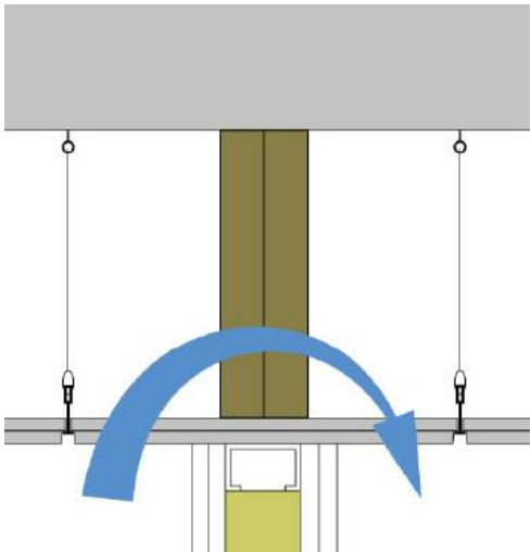
Fig 1. Sound Transmission Path
