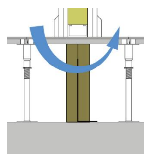
Fig 5 Access floor void cross-talk path
