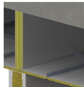
Fig 2. Friction fit in a low height void
