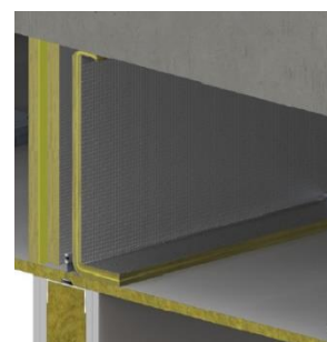
Fig 4. Twin barrier using CVB & CBX
