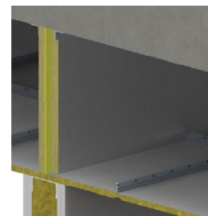
Fig 3. Head fixing with twin angles
