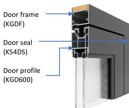
Kross Glaze Door and Frame
