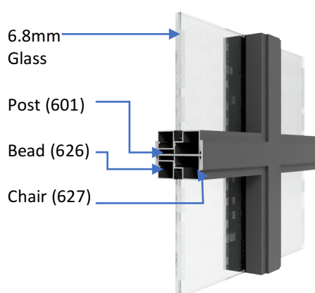
Kross Glaze Single Glazed
