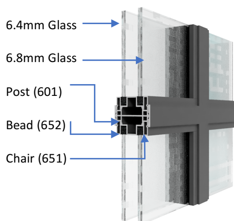
Kross Glaze Double Glazed
