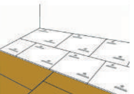
5. Check the subfloor is free from debris and completely flat. Minor differences in levels can be evened out by spreading a thin layer of tile adhesive on to the subfloor. Fix the 6mm Multi-pro Tile Backer board to the floor at 200mm fixing centres using countersunk screws.
