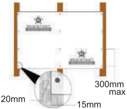
3. 9 & 12mm Multi-pro Tile Backer for walls. Space fixings minimum 20mm from bottom & 15mm from side at 300mm intervals. Ensure screws are countersunk.
